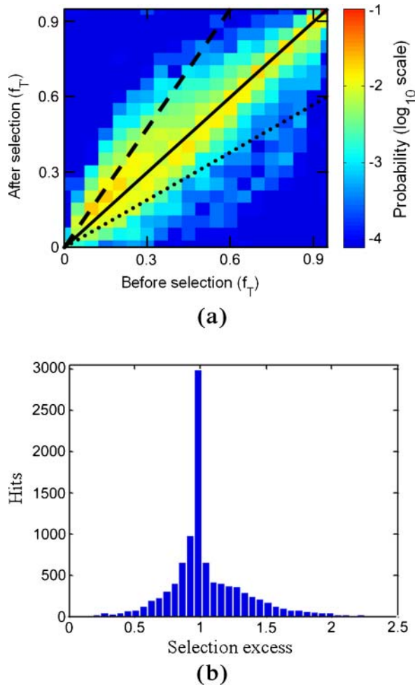
Figure 2. Selection in GARD. (a) The correlation between the frequencies of the target comptype in the basal simulation ( f_T ) and its frequency after applying selection ( f_T ). In the electronic version, color represents probability out of the entire data set of 10,000 simulations, and positive and negative selection are respectively seen above and below the diagonal (selection excess = 1.0, solid black line). The dashed and dotted lines respectively mark selection excesses of \frac{3}{2} and \frac{1}{2} . (b) Selection excess histogram for the entire data set. Simulation parameters are given in Table 1.
