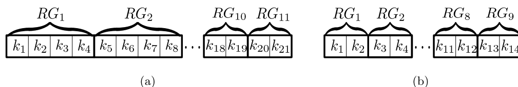
Figure 7. The structure of the chromosome holding the rate constants of (a) the weight-loop perceptron, (b) the weight-race perceptron. The rate constants (chromosome elements) are shared among reactions within the reaction group (RG) as defined in Table 3.
