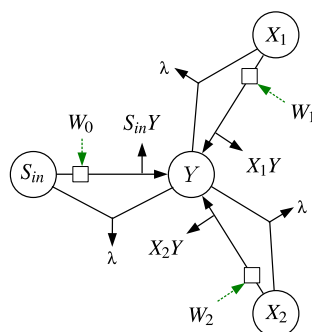
Figure 1. Reactions in the input-weight integration of a two-input AASP. Dotted arrows denote a catalyst, for example, signifying X_i \xrightarrow{W_i} Y + X_i . Each weight catalyzes a reaction turning its associated input into Y , while that input and Y simultaneously annihilate each other at a different rate. Reproduced from our article on the AASP [4].
