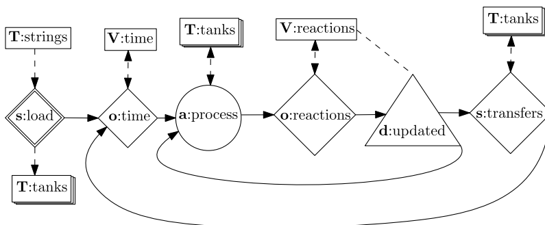
Figure 6. Macro-level description of (open-ended) StringCatChem.
