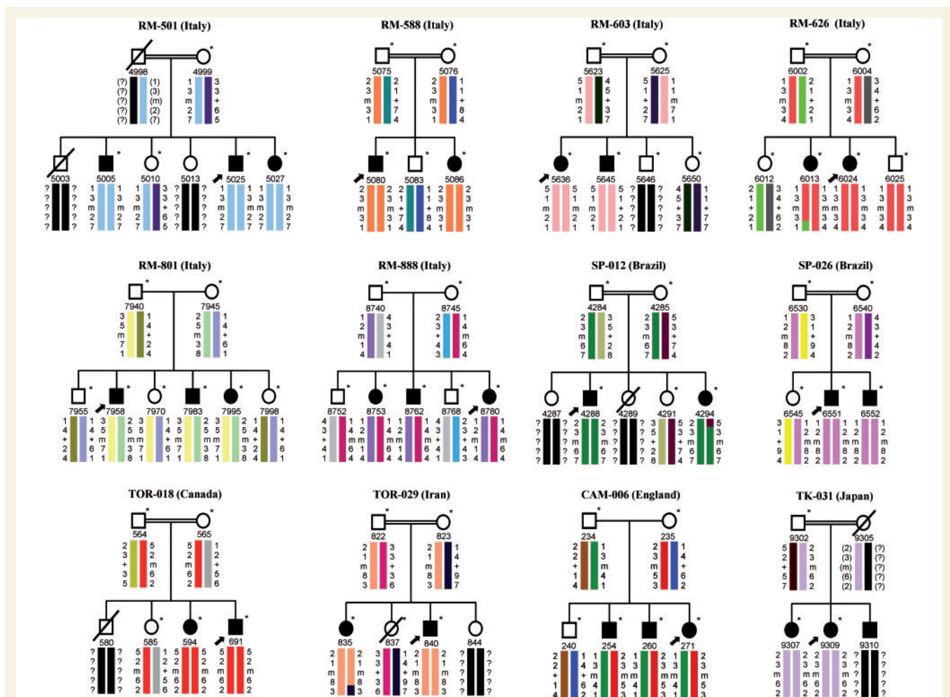
Figure 1 Pedigrees and segregation chart of 12 ARCMT2 families linked to the ALS5/SPG11 locus. Black solid symbols indicate affected individuals carrying ALS5/SPG11/KIAA1840 mutations; white symbols represent unaffected subjects; square symbols are males, circles are females, and slashed symbols are deceased individuals. Individuals are reported as code numbers below the symbols. Probands are marked by arrows. Colour barcodes define the haplotypes created with markers D15S146, D15S537, D15S659, and D15S123, from top to bottom. Reconstructed genotypes are indicated by parentheses and question marks symbolize alleles that could not be reconstructed. The ALS5/SPG11/KIAA1840 gene is placed between markers D15S537 and D15S659; key recombination events are observed between markers D15S659 and D15S123 in Patients 6013 (Family RM-626) and 835 (Family TOR-029), as well as between markers D15S146 and D15S537 in Patient 4294 (Family SP-012). * = sample subjects; m = mutation; + = wild-type.
