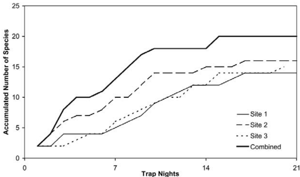
Figure 4. Species accumulation curves for pitfall and Elliott trapping at each of the three trap sites in the Little Desert National Park. Data from all trapping sessions has been combined to create the curves.
