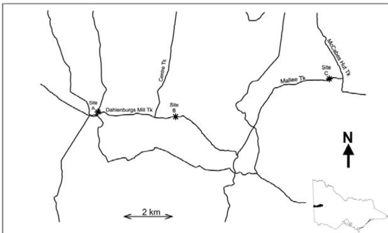
Figure 1. Location of trapping sites in the eastern block of the Little Desert National Park. Inset map shows location of the Little Desert National Park in Victoria.
