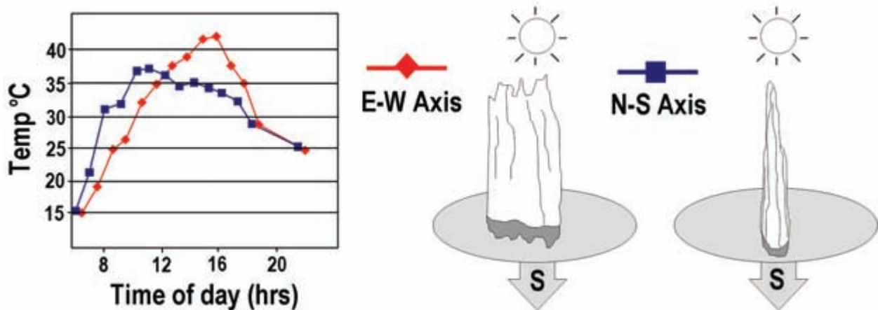
Figure 3. The effect of a 90° rotation on the core temperature, averaged over 3 days in both orientations, of an A. Laurensis mound in the north Australian dry season (modified from Grigg 1973).
