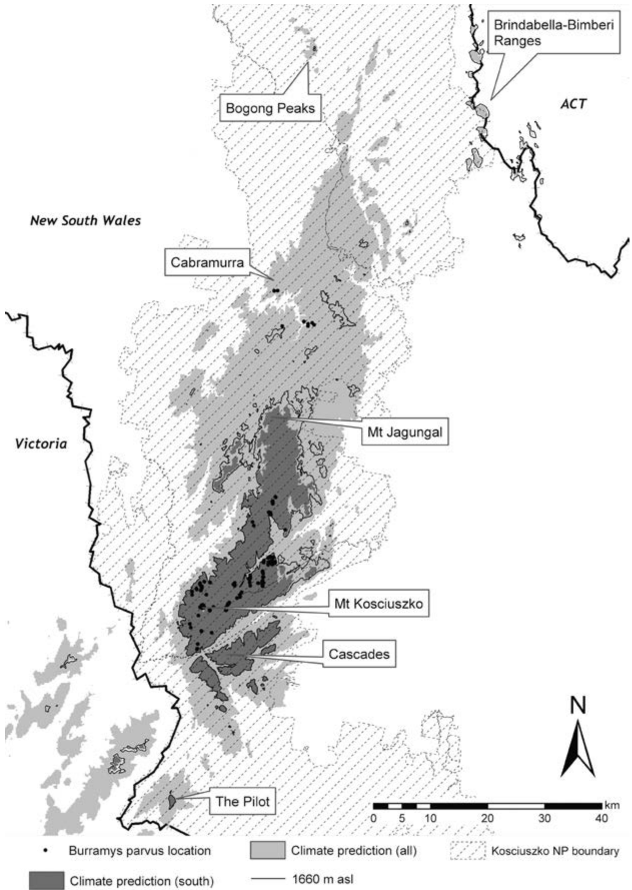
Figure 4. Climatic predictions based on known populations of Burrumys parvus in NSW. The “south” prediction is based on populations studied in the survey component of this study, the “all” prediction includes the recently discovered northern population.
