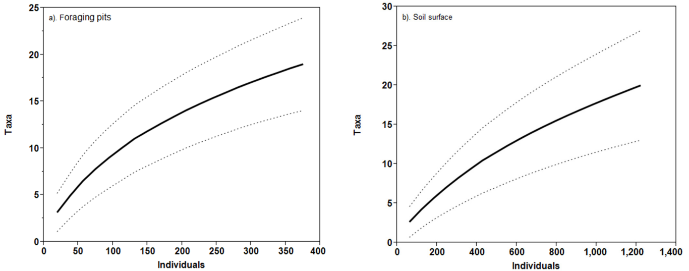
Figure 2. Comparison of individual rarefaction curves for ants trapped in a). foraging pits and b). on the soil surface shown with 95% confidence intervals.
