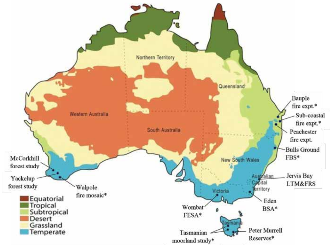
Figure 1. Location of long-term fire study sites within temperate and sub-tropical forests. * indicates sites with an invertebrate component.
