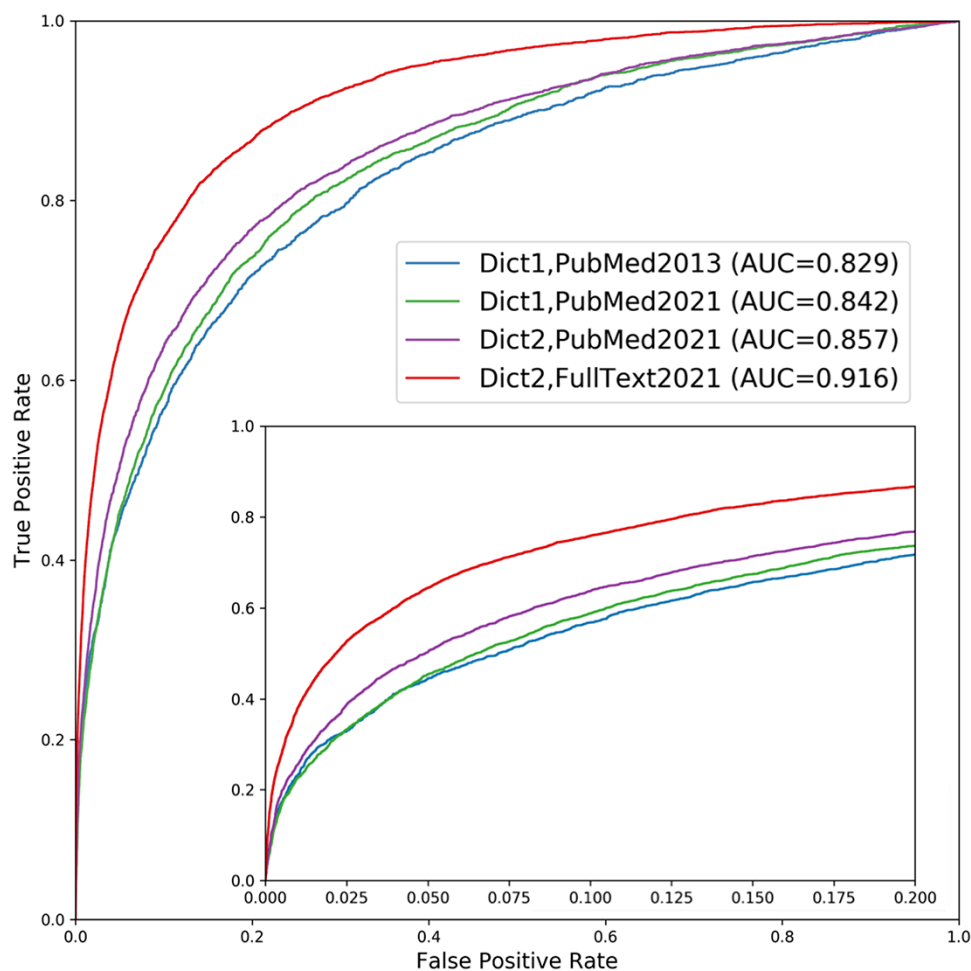
Figure 2. Performance improvement of the text mining channel. As shown in the ROC curves, text mining performs markedly better in the new version of DISEASES (Dict2, FullText2021) compared to the originally published one (Dict1, PubMed2013). To quantify the sources of improvements, we show two additional curves: one using the new dictionary on the latest abstract collection only (Dict2, PubMed2021) and another using the old dictionary on the same abstracts (Dict1, PubMed2021). Comparing the curves reveals that most of the improvement stems from the addition of full-text articles, but that the new disease and gene dictionaries also led to considerable improvement. By contrast, the growth in PubMed abstracts from 2013 to 2021 made only a minor difference. The insert shows a zoom of the high-confidence part of the plot.
