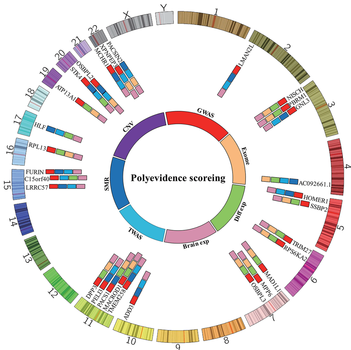
Figure 2. Top candidate causal genes identified in this study. By integrating prediction results from different methods, 29 high-confidence causal genes were identified. OSBP2L, STK4 and PACS1 had the highest scores and thus represent the most promising causal genes for BIP.
