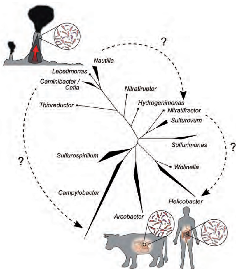
Figure 2. Phylogenetic tree showing the position of cultured pathogenic and environmental strains of the Epsilonproteobacteria. Two hypothetical patterns of gene flow from thermophilic geothermal strains (top left) to commensal and pathogenic strains (bottom) are shown.
