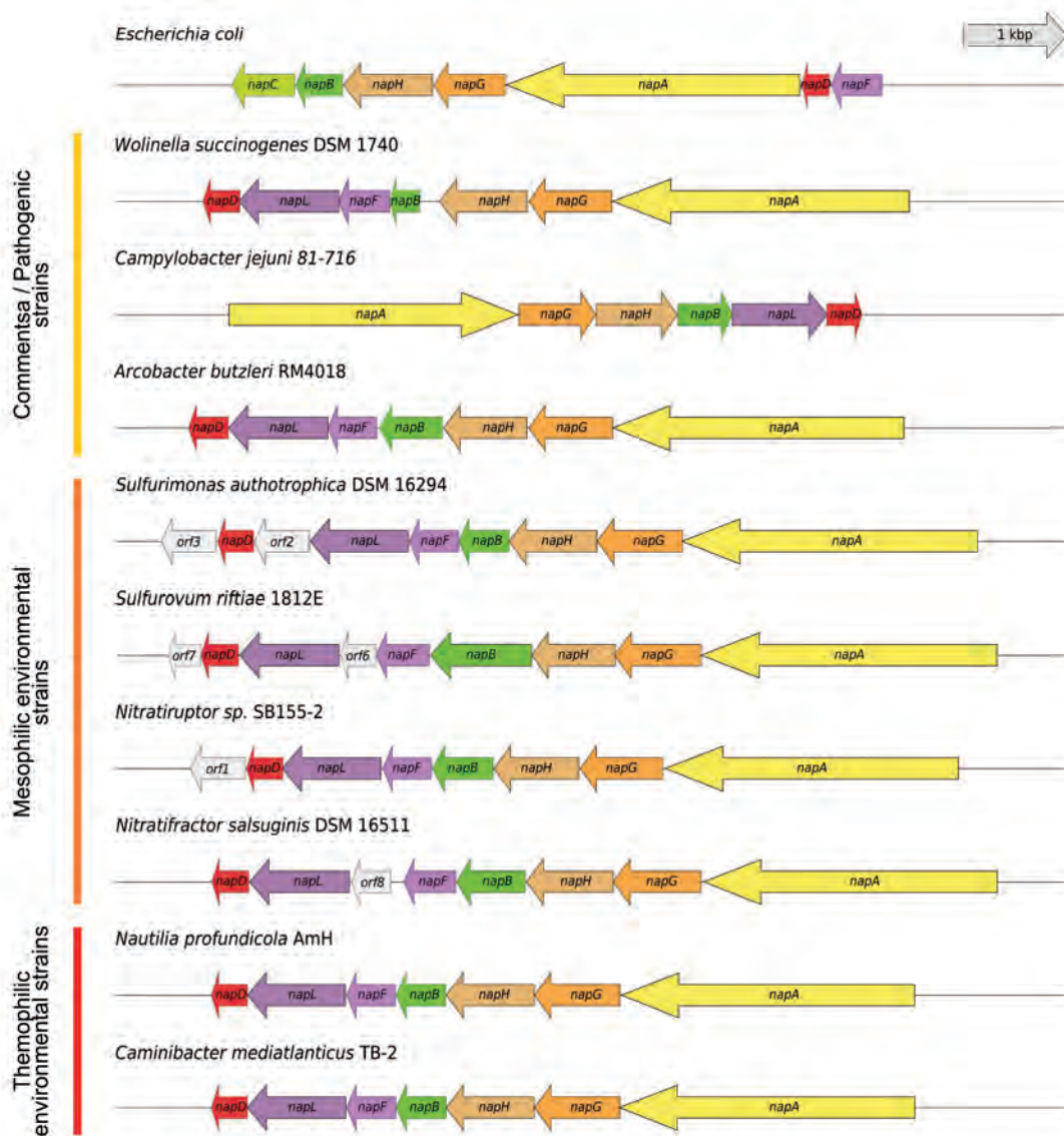
Figure 4. The conserved periplasmic nitrate reductase (Nap) operon structure in pathogenic and environmental Epsilonproteobacteria . The ability to respire nitrate using high affinity enzymes such as the periplasmic nitrate reductase appears to be a conserved strategy in colonizing deep-sea vents and the human gastrointestinal tract. The nap cluster in Escherichia coli is included as a reference.
