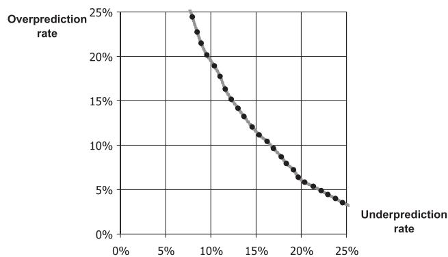
Fig. 4. The curve of overprediction rate ( E_2 ) versus underprediction rate ( E_1 ).
