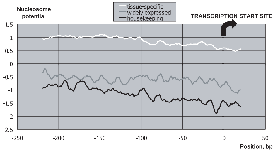
Fig. 7. Average nucleosome formation potential \varphi(X) profiles of gene promoters of different expression classes.
