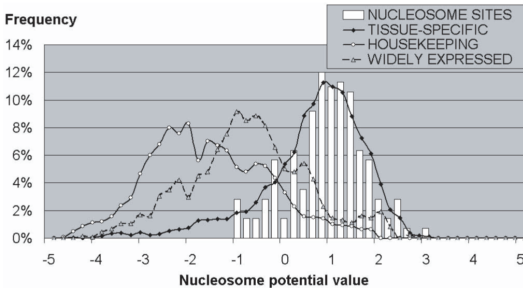
Fig. 8. Histogram of the nucleosome formation potential \varphi(X) distributions for gene promoter regions (for comparison, see the distribution of the training set of nucleosome sites): promoters of housekeeping genes, promoters of genes expressed in various tissues, and promoters of tissue-specific genes.
