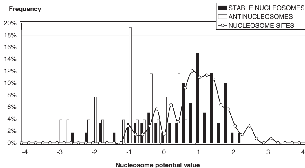
Fig. 6. Histogram of nucleosome formation potential \varphi(X) distributions for the sequence sets of high and low affinity to histone octamer in comparison to distribution \varphi(X) for the set of nucleosome sites.
