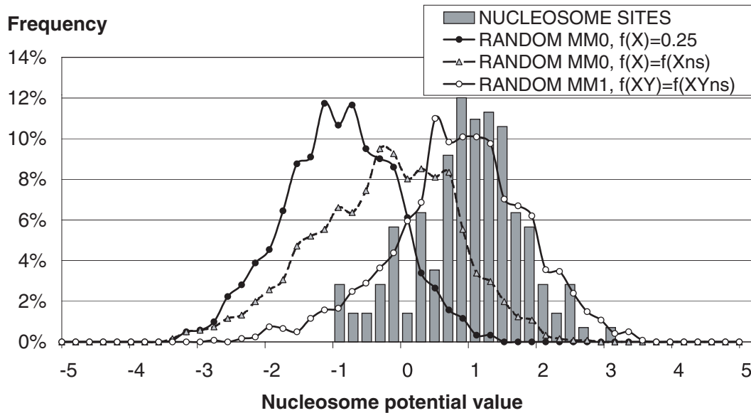
Fig. 5. Histogram of nucleosome formation potential \varphi(X) distributions for randomly generated samples of sequences in comparison to distribution \varphi(X) for the set of nucleosome sites: (1) nucleotide frequencies equal to 0.25; (2) and (3), the sequences are generated by the set of nucleosome sites with conservation of the mono- and dinucleotide content. MM0 is Markov model of order 0; MM1, of order 1. f(Xns) and f(XYns) denote mono- and dinucleotide frequencies of nucleosome site sequences.
