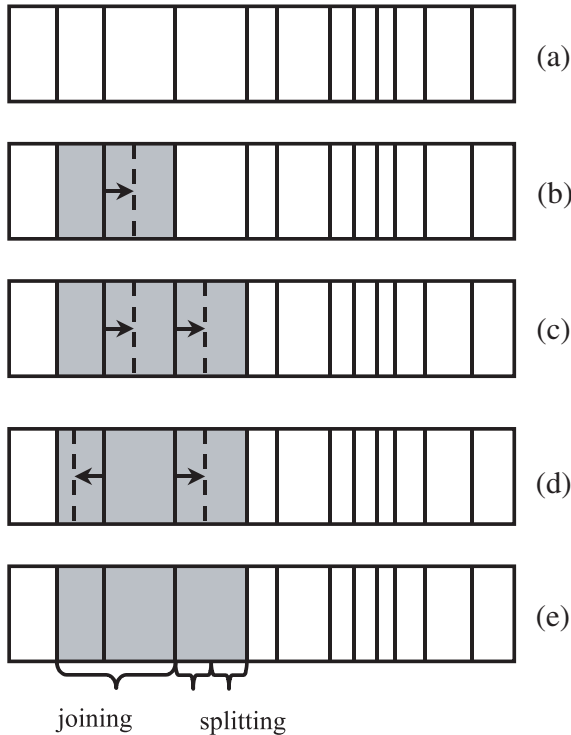
Fig. 2. Examples of modifications used by the algorithm searching for optimal partition: (a) arbitrary distribution; (b) shift of the border between adjacent regions; (c) shift of a region relative to the neighbouring regions; (d) symmetrical shift of the region's borders relative to its centre; and (e) joining and splitting.
