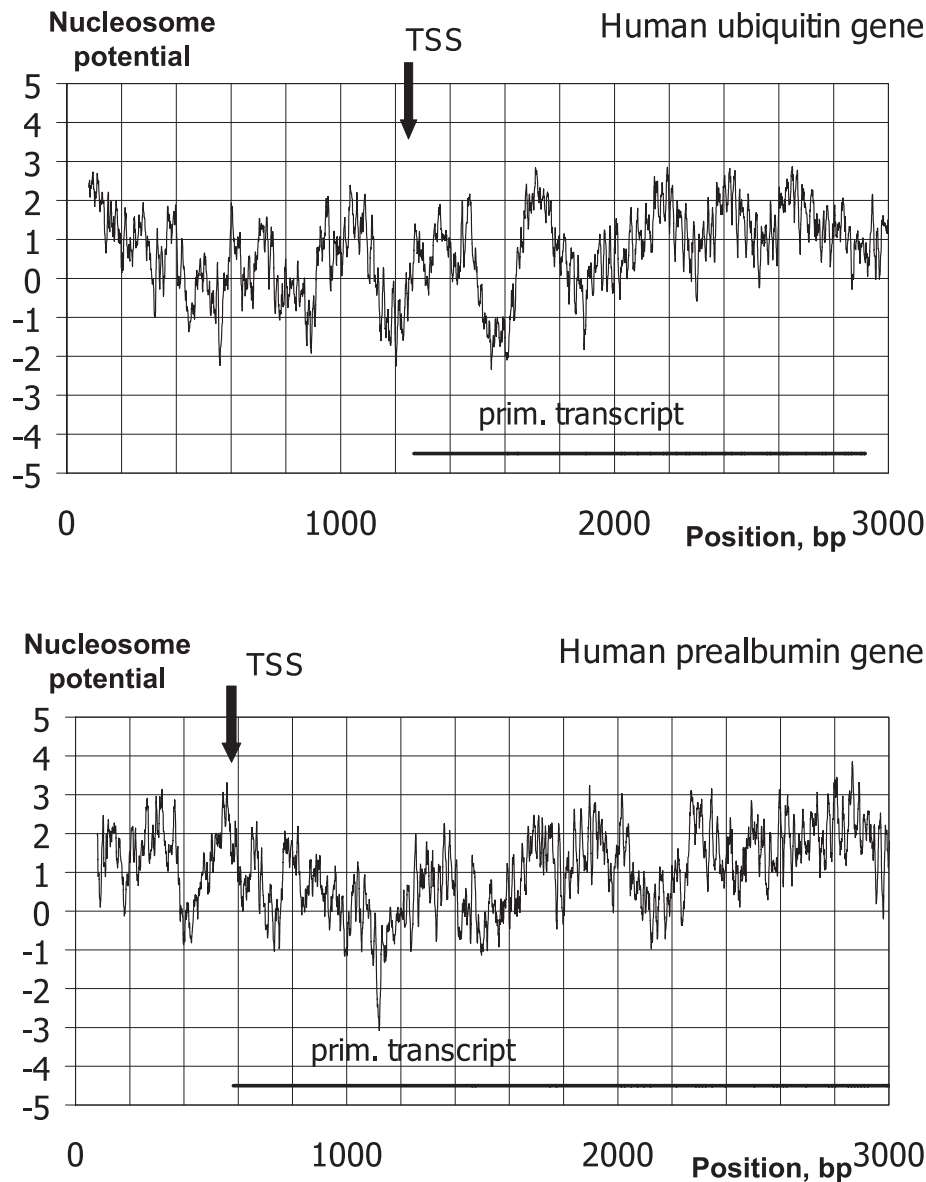
Fig. 9. Nucleosome formation potential \varphi(X) profiles for housekeeping ubiquitin gene (AC U49869) and tissue-specific prealbumin gene (AC M11844). TSS—Transcription Start Site, primary transcript locations are shown below.
