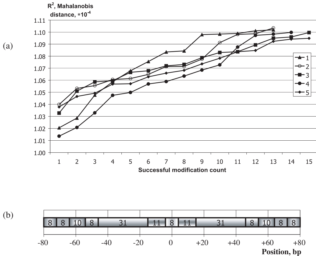
Fig. 3. (a) Growth dynamics of Mahalanobis distance R^2 , five optimization cycles are presented; (b) partitions of the entire nucleosome site region [-80; +80] used for constructing nucleosome formation potential profile.
