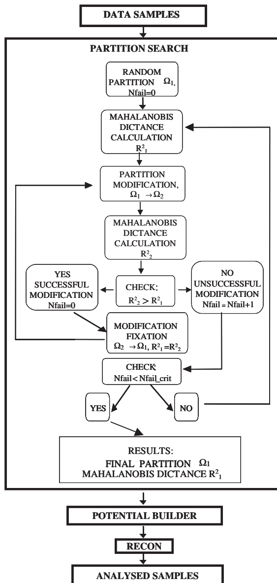
Fig. 1. Basic components of the system NucleoMeter (bold type) and scheme of the algorithm constructing the nucleosome formation potential profile (block PartitionSearch).
