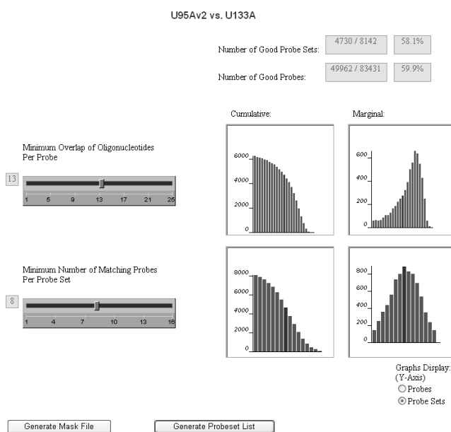
Fig. 1. The mask file generation page of http://www.crosschip.org . The user generates mask files for the two chip types to be compared, according to the criteria on the minimum sequence overlap length and the minimum number of probe pairs per probe set.
