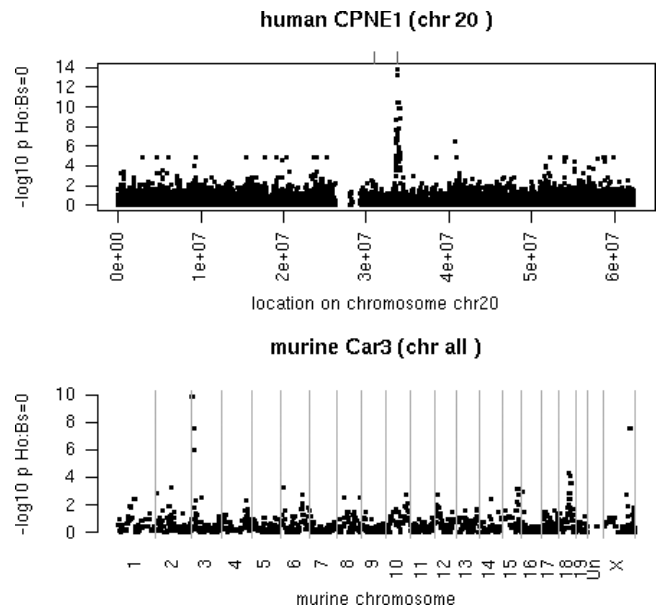
Fig. 1. Illustration of cis -acting determinants on human chromosome 20 for expression of CPNE1 (upper), and on complete BXD murine genome for expression of Car3 (lower). For the model \log CPNE1 = \alpha_s + \beta_s X_s + e_s , the null hypotheses H_0: \beta_s = 0 are tested using the t statistic with X_s denoting the number of copies of the minor allele for SNP s . The y-axis plots (nominal) negative \log_{10} p for these hypotheses; the x-axis are chromosomal locations of SNPs s .
