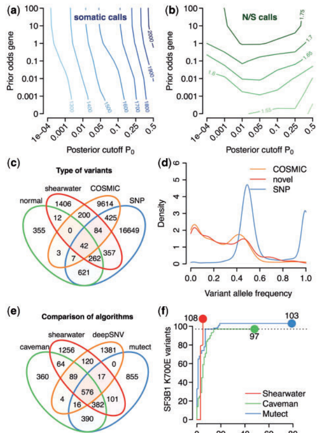
Fig. 3. Variants in MDS. (a) Number of non-polymorphic variant calls versus cutoff P_0 and prior weight \pi_{\text{gene}}/(1 - \pi_{\text{gene}}) . (b) Ratio of non-silent to silent variant calls. (c) Venn diagram of the distribution of shearwater variants across a normal panel, known SNPs and COSMIC variants. (d) Distribution of variant allele frequencies. (e) Venn diagram of calls from different algorithms. (f) Number of SF3B1 K700E calls as a function of false positives for different variant callers
