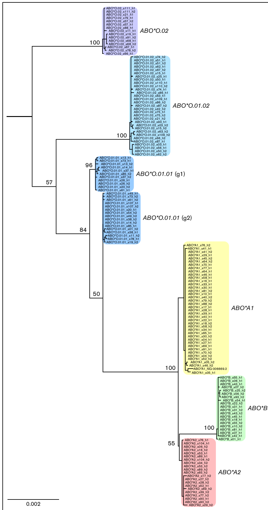
Figure 3. Maximum-likelihood phylogenetic tree based on the entire ABO gene locus. All ABO groups form distinct evolutionary clades with an additional split of ABO *O.01.01 into 2 subgroups (g1 and g2). Bootstrap support is provided for main branching points. The tree was rooted with central chimpanzee sequence (not shown).
