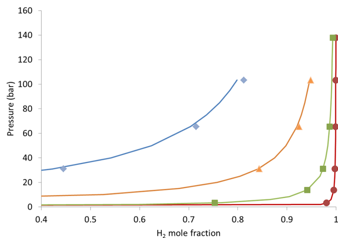
Fig. 6. Experimental data and computed dew curves for the system H 2 + H 2 O. Symbols: experimental data (Gillespie and Wilson, 1980) at 310.93 K (circles), 366.48 K (squares), 422.04 K (triangles) and 477.59 K (diamonds). Solid lines: SW equation of state.
