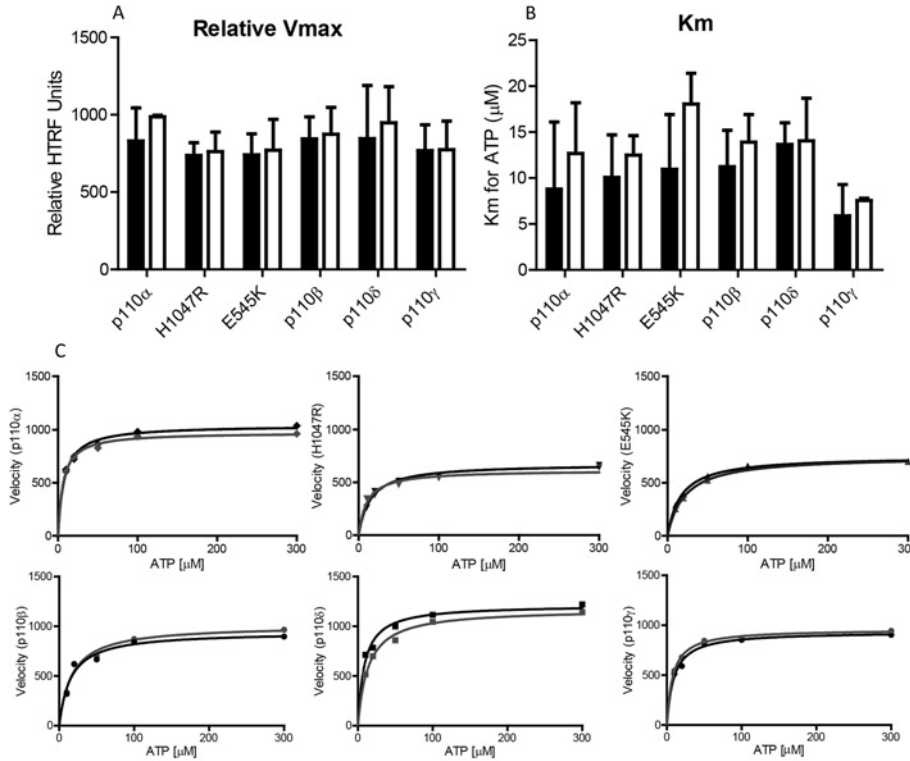
Figure 2 Kinetic analysis of His-tag (solid bars) and His-tag-free (open bars) kinases as labelled (median ± range, n \geq 2 ) (A) Relative V_{max} , (B) K_m for ATP in \mu M , (C) Representative Michaelis–Menten plots for all kinases as detailed on y-axis (His-tag, black line; His-tag-free, grey line).
