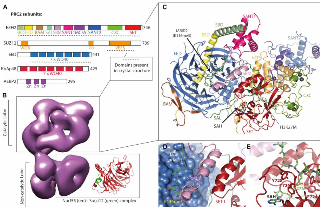
Figure 3. The PRC2.
