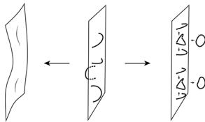
D-brane
