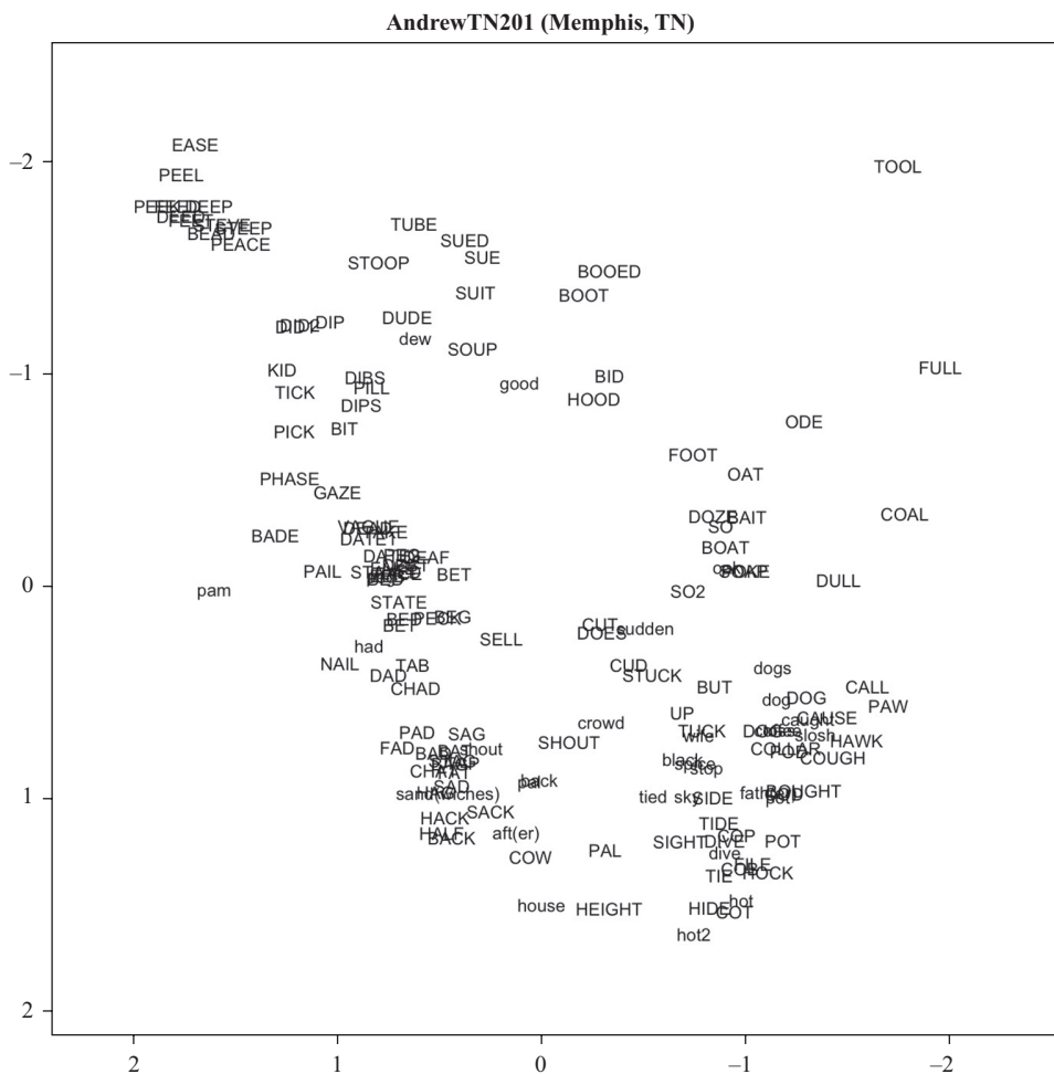
Figure 18.1 Example vowel plot showing one-third measurement point for 155 vowel tokens for participant AndrewTN201 (male from Memphis, Tennessee, between thirty-one and forty years old). Data are Lobanov normalized (Kendall & Thomas 2010).
