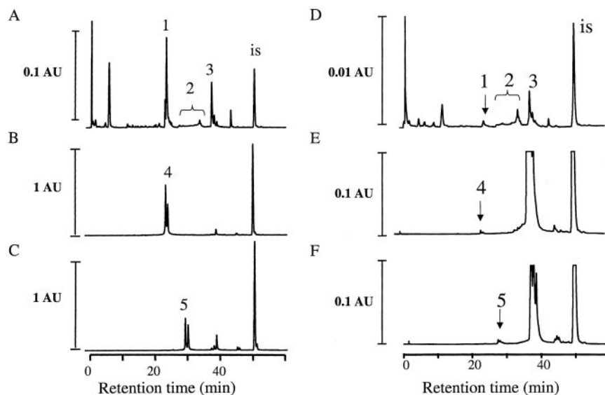
Fig. 2. High-performance liquid chromatograms of extracts of incubations of curcumin (100 \mu M) with cytosol (A and C) and microsomes (B) from human intestinal tissue and with cytosol (D and F) and microsomes (E) from rat intestinal tissue. Incubation periods were 90 min for metabolic reduction (A and D) and 60 min for conjugation (B, C, E, and F). Chromatographic analysis was conducted with detection at 280 (A and D) and 420 nm (B, C, E, and F). The identity of the peaks was established by cochromatography and mass spectrometry as curcumin (peak 3), hexahydrocurcumin (1), tetrahydrocurcumin (2), curcumin glucuronide (4), and curcumin sulfate (5). The prominent peak labeled "is" (retention time: 51 min) was caused by the internal standard 5,10,15,20-tetra-( m -hydroxyphenyl)-chlorine. Note that commercially available curcumin contains 15% desmethoxycurcumin and 5% bisdesmethoxycurcumin, which furnished two small peaks just beyond curcumin (see especially in A and D). Removal of the methoxy moieties from the curcumin molecule appears to render its phenolic groups more resistant against metabolic conjugation, and bisdesmethoxycurcumin was not a substrate of the conjugating enzymes. AU, absorbance units. For details of incubation, extraction, and HPLC analysis, see "Materials and Methods." The chromatograms are representative of analyses conducted with fractions or tissues from three humans or four rats.
