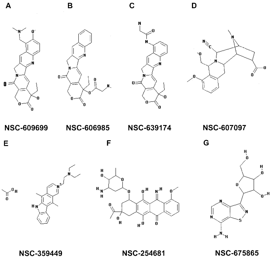
Fig. 4. Chemical structures of positive hits. A, NSC-609699, topotecan. B, NSC-606985, camptothecin, 20-ester(S). C, NSC-639174, 9-glycineamido-20(S)-camptothecin HCl. D, NSC-607097, DX-52-1, quincarmycin analogue. E, NSC-359449, 2-(5,11-dimethyl-6H-2λ 5 -pyrido[4,3-b]carbazol-2-yl)-N,N-diethylethanamine acetate. F, NSC-254681, 3-acetyl-3,5,12-trihydroxy-11-imino-10-methoxy-6-oxo-1,2,3,4,6,11-hexahydro-1-naphthacenyl 3-amino-2,3,6-trideoxyhexopyranoside. G, NSC-675865, 1-(7-aminoisothiazolo[4,5-d]pyrimidin-3-yl)-1,4-anhydrosorbitol.
