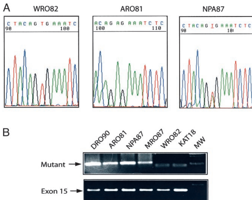
Fig. 1. BRAF gene mutation analysis in thyroid tumor cell lines. A , DNA sequencing. Genomic DNA from 10 thyroid tumor cell lines was extracted and used as a template to amplify a DNA fragment flanking exon 15. The amplified PCR product was sequenced with a forward primer to amplify exon 15 of the BRAF gene. Three sequences representing the wild-type BRAF gene (WRO81), homozygous/hemizygous BRAF mutation (ARO81), and heterozygous BRAF mutation (NPA87) are shown. B , MASA analysis of BRAF gene mutation in thyroid tumor cell lines. Genomic DNA samples of 6 representative thyroid tumor cell lines were used as templates in PCR reactions to specifically amplify mutant BRAF gene by using a mutant-specific primer. Exon 15 was amplified as a positive control by using two intron primers flanking it. The PCR conditions were 94°C, 2 min (94°C 30", 52°C 45"; 72°C 45") × 35 cycles; 72°C, 8 min. PCR products were analyzed in a 3% agarose gel and stained with ethidium bromide.
