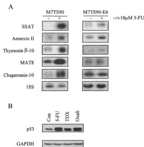
Fig. 2. A , Northern blot analysis of SSAT, annexin II, thymosin \beta -10, MAT-8, and chaperonin-10 mRNA expression in p53 wild-type M7TS90 cells and p53-null M7TS90-E6 cells treated for 72 h with no drug (-) or 10 \mu M 5-FU (+). 18S rRNA was assessed as a loading control. B , Western blot analysis of p53 expression in MCF-7 cells treated for 72 h with no drug (Con) or IC 60 s of 5-FU, TDX, or oxaliplatin (Oxali). Glyceraldehyde-3-phosphate dehydrogenase expression was assessed as a loading control.
