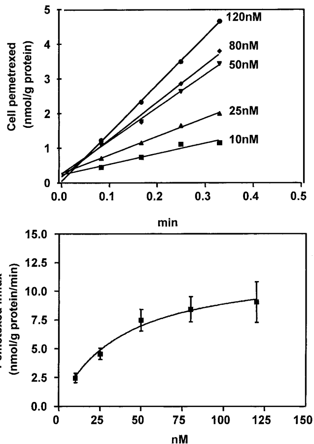
Fig. 2. The kinetics of [ ^3\text{H} ]pemetrexed influx in NCI-H28 cells. Top panel , initial uptake over the concentration range studied, on which rates were computed as indicated in the bottom panel . Bottom panel , pemetrexed influx as a function of the extracellular concentration. The data are the average of three experiments.
