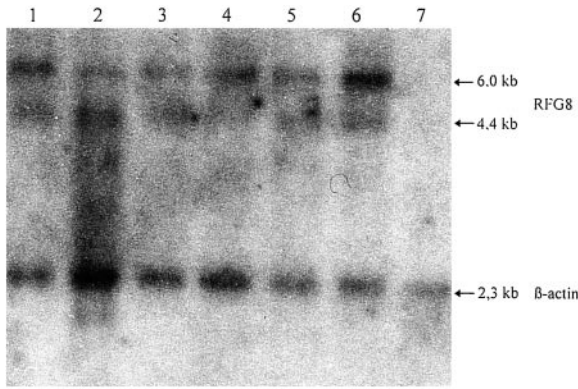
Fig. 2. Expression of RFG8 mRNAs as seen by Northern blot analysis of various tissues. The tissues used are as follows: 1, stomach; 2, thyroid; 3, spinal cord; 4, lymph node; 5, trachea; 6, adrenal gland; and 7, bone marrow. We detected messages of about 6.0 and 4.4 kb in length in all of the tissues tested except in the bone marrow.
