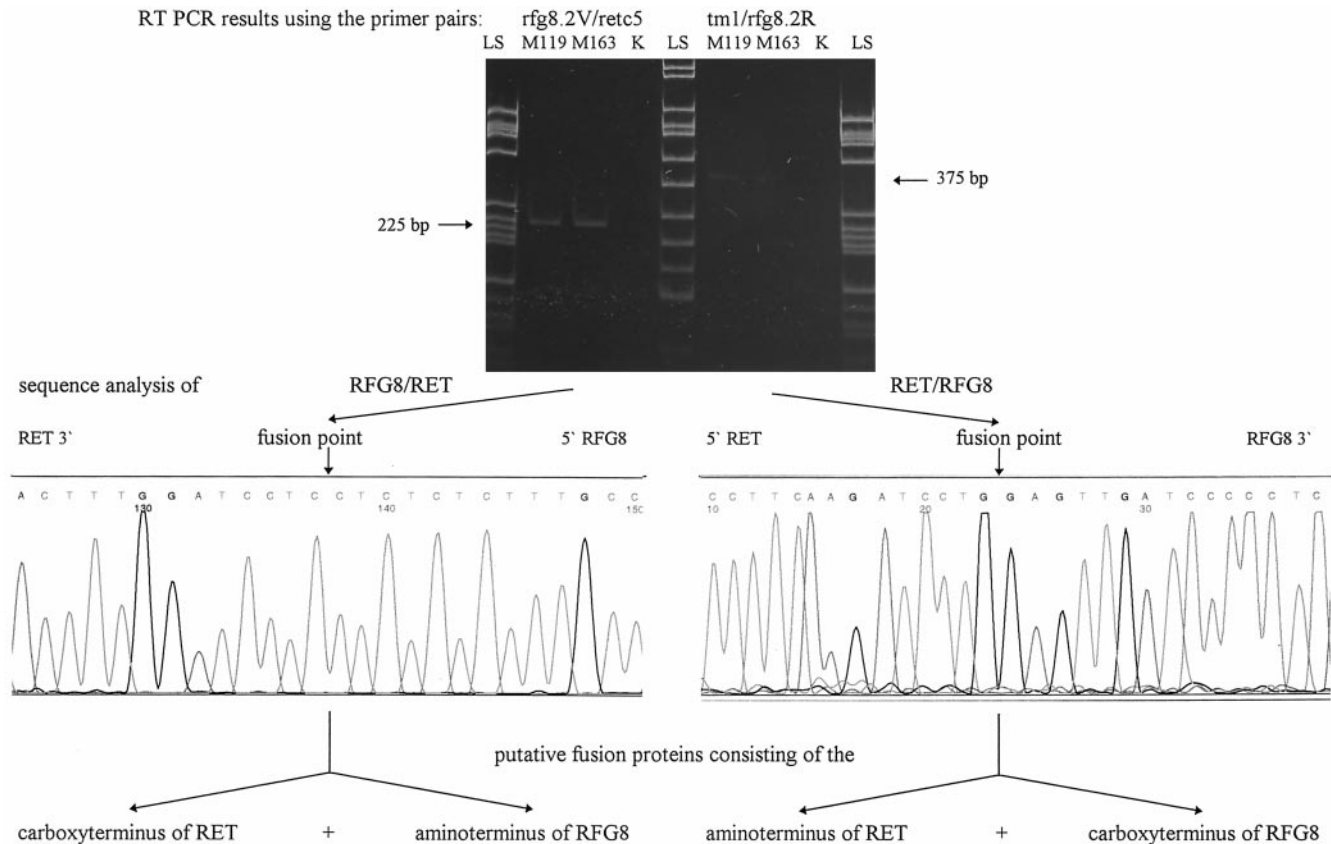
Fig. 1. Results of RT PCR and the corresponding sequencing analysis to identify the PTC8 rearrangement in tumor samples M119 and M163. The PTC8 rearrangement consists of two chimeric transcripts designated RFG8/RET and RET/RFG8. The direction of the sequence analysis is 3' to 5' for RFG8/RET and 5' to 3' for RET/RFG8. The corresponding fusion points are indicated by arrows. The RET part of the RET/RFG8 sequence ends with nucleotide 1334, whereas the RET portion of the RFG8/RET sequence starts with nucleotide 1335 of the RET cDNA sequence (37).
