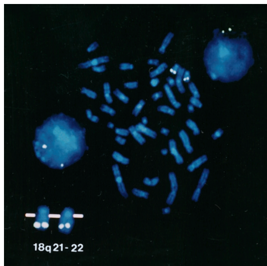
Fig. 4. Digitized pseudocolored images of human metaphase chromosome 18 after FISH of PAC RPCIP704B06764Q2. The similar result obtained using PAC RPCIP704H1212Q25 is not shown. The hybridization signals of both PACs were mapped to chromosome 18q21–22.
