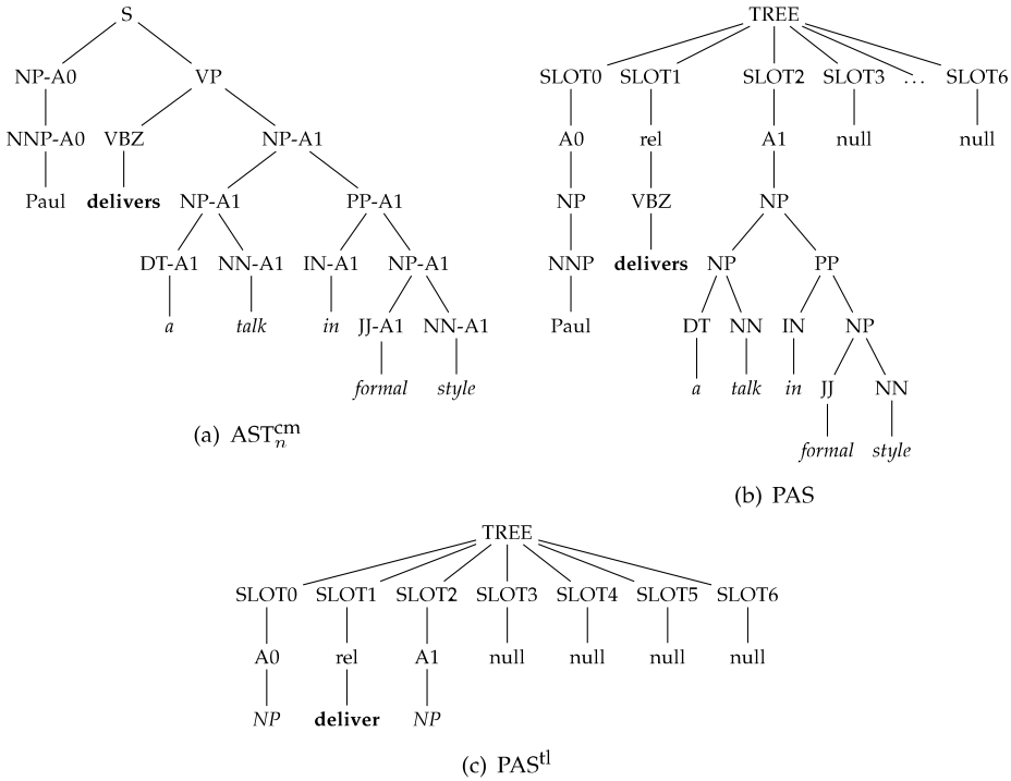
Figure 8 Different representations of the same proposition.
