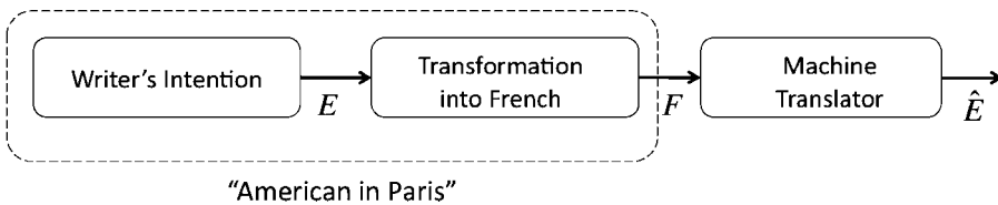
Figure 4 Schematic of statistical machine translation.
