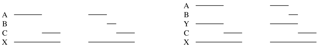
Figure 17 Left, example spans for a ternary rule decomposition \mathcal{X} \rightarrow \mathcal{A}\mathcal{B}\mathcal{C} . Each symbol represents a subset of nonterminals from the original SCFG rule, and the subsets may cover discontinuous spans in either language. Line segments represent the projection of each set of child nonterminals into a single language, as in Figure 15. Right, factorization into \mathcal{X} \rightarrow \mathcal{Y}\mathcal{C} and \mathcal{Y} \rightarrow \mathcal{A}\mathcal{B} .
