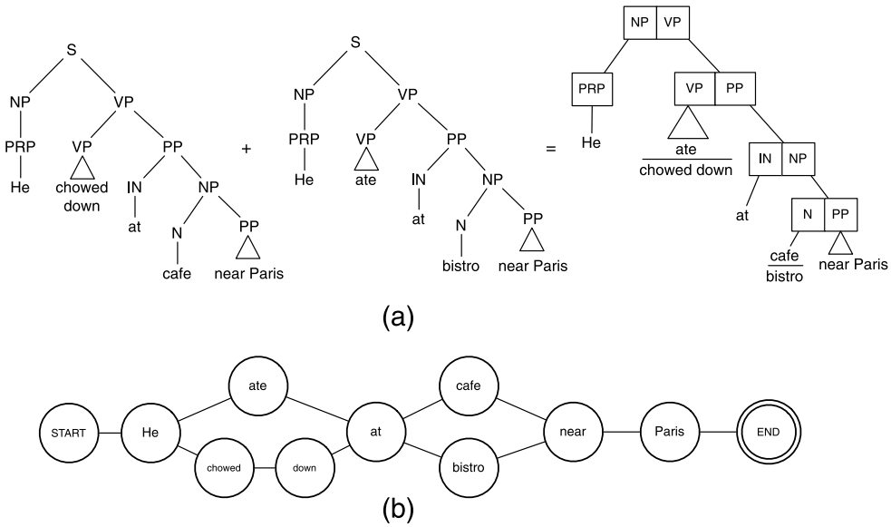
Figure 5 The merging algorithm. (a) How the merging algorithm works for two simple parse trees to produce a shared forest. Note that for clarity, not all constituents are expanded fully. Leaf nodes with two entries represent paraphrases. (b) The word lattice generated by linearizing the forest in (a).
