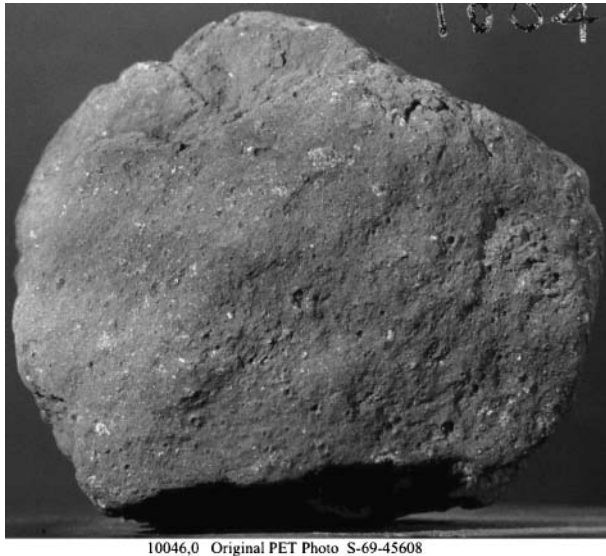
Figure 1 A photograph of lunar rock, sample 10046.
