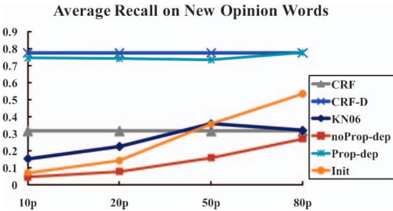
Figure 5 Recalls of Init, CRF, CRF-D, KN06, noProp-dep, and Prop-dep.
