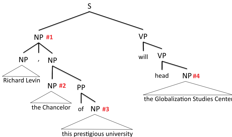
Figure 2 Example of left-to-right breadth-first tree traversal. The numbers indicate the order in which the NPs are visited.
