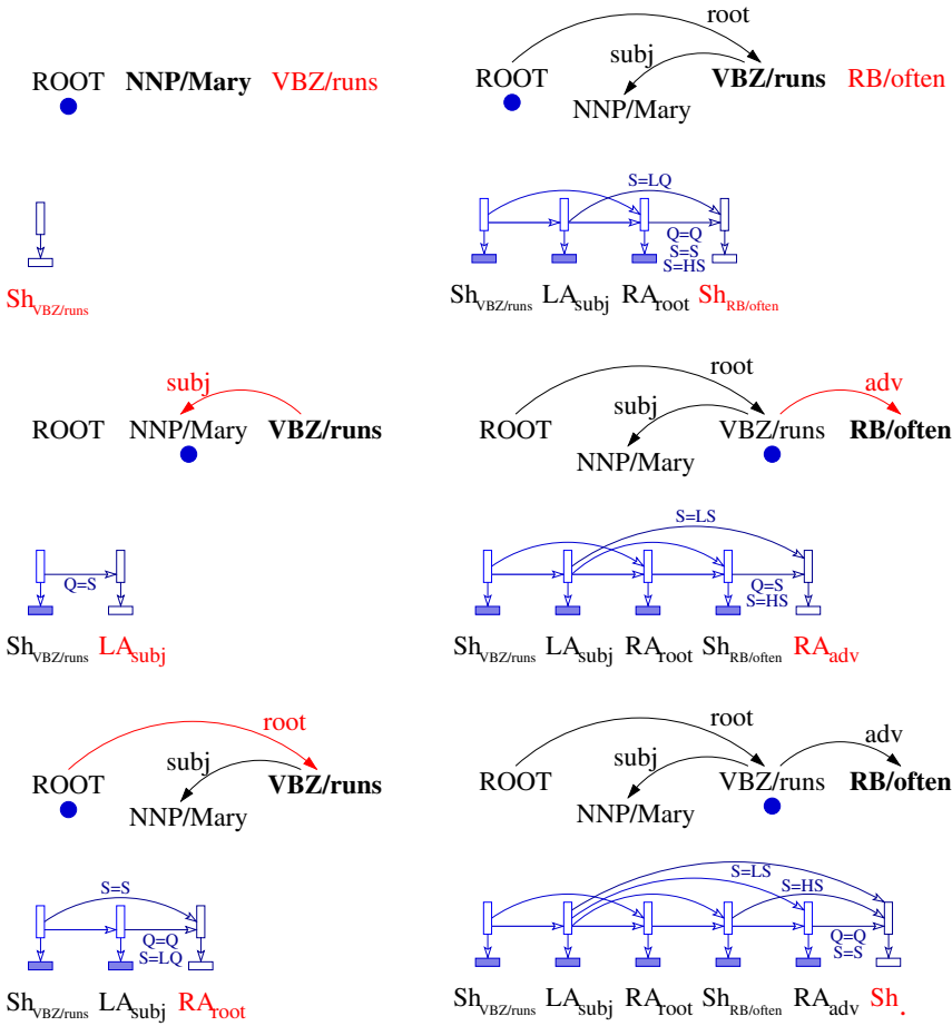
Figure 8 Illustration of the derivation of a syntactic output structure and its associated incremental specification of an ISBN model structure (ordered top-to-bottom, left-to-right). The blue dot indicates the top of the syntactic derivation’s stack and the bold word indicates the front of the input queue. New model structure edges are labeled with the relationship between their source state and the current state, respectively, with Q for queue front, S for stack top, HS for head of stack top, LQ for leftmost child of queue front, and LS for leftmost child of stack top.
