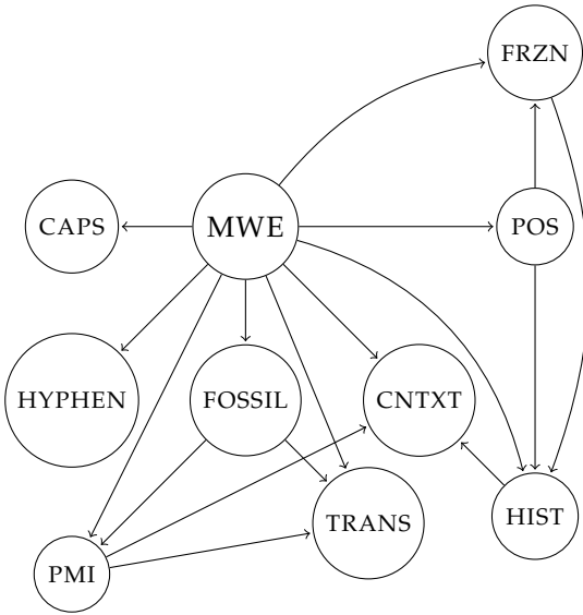
Figure 1 The Bayesian network for MWE identification.
