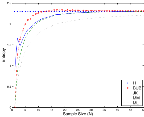
Figure 1 The estimated and true entropy for uniform distribution.
