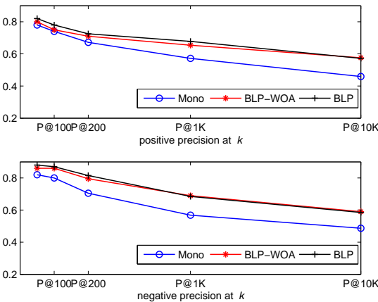
Figure 3 Precision evaluation of the experiments based on monolingual (Mono), bilingual without antonym (BLP-WOA), and bilingual (BLP) word graphs.
