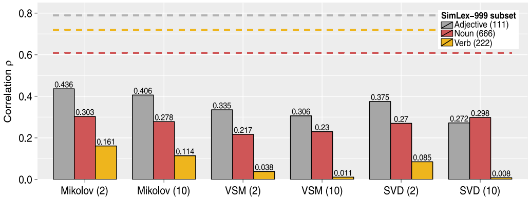
Figure 11 Performance of models on POS-based subsets of SimLex-999. The window size for each model is indicated in parentheses. Inter-annotator agreement for each POS is indicated by the dashed horizontal line.
