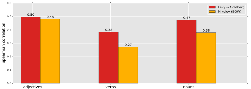
Figure 12 The importance of dependency-focused contexts (in the Levy & Goldberg model) for capturing concepts of different POS, when compared to a standard Skipgram (BOW) model trained on the same Wikipedia corpus.
