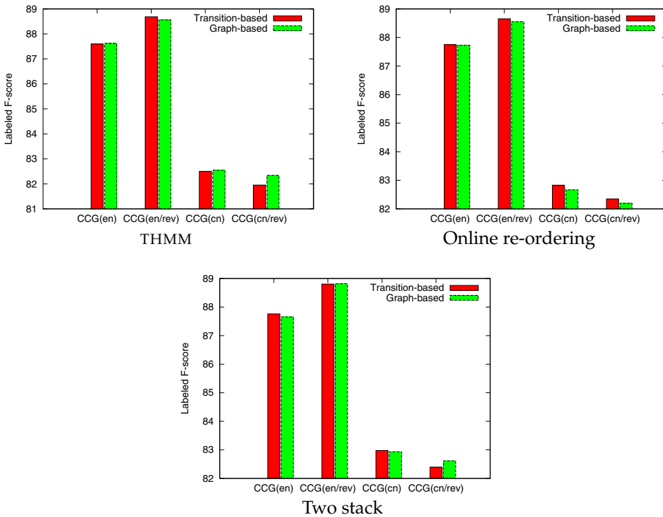
Figure 12 Labeled F-scores with respect to different tree parsing techniques. Results shown here are from experiments for English and Chinese CCG parsing.
