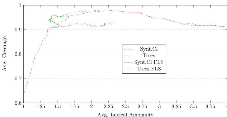
Figure 4 Coverage with respect to averaged lexical ambiguity. Data points are obtained from the different configurations, with/without FLS and n -best sequences with n = 1 \dots 20 ; except for the Trees without FLS, where the results include up to n = 70 configuration.
