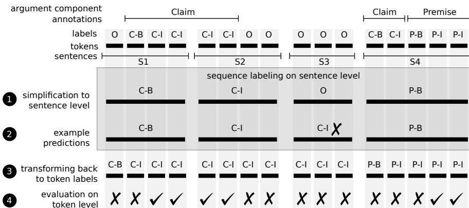
Figure 8 Our approach to simplifying argument component segmentation and evaluation of the system. Gold data are labeled on the token level ( C = Claim , P = Premise ). In step 1, the argument component label becomes a new label for the entire sentence. The resulting label reflects if the component begins in the sentence (i.e., the case of Claim-B in S1 ). If there are more components in one sentence, the longest one is selected (i.e., the case of Claim and Premise in S4 ). In step 2, the predictions are obtained for entire sentences, as one sentence represents the minimal unit in sequence labeling mode. In step 3, the labels are translated back to the token level, spanning over the entire sentence. If the predicted label is a *-B tag, the first token is labeled as *-B and the remaining ones as *-I (i.e., in S1 and S4 ). In step 4, evaluation of predictions is performed solely on the token level by comparing the predicted token labels with the gold token labels.
