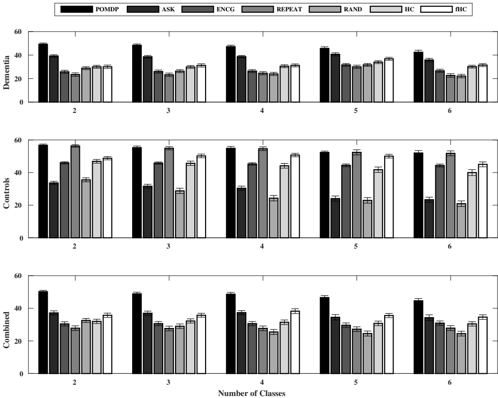
Figure 9 Mean number of accumulated rewards in learned POMDP policies, and the baseline policies.
