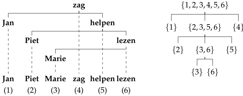
Figure 12 A dependency structure and the recursive partitioning extracted from it by Algorithm 3.
