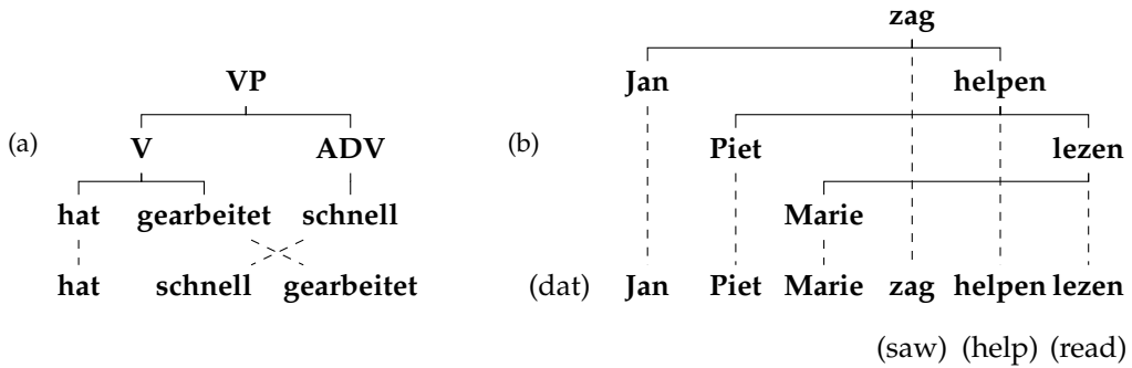
Figure 4 (a) Discontinuous phrase structure for German “[...] hat schnell gearbeitet” (“[...] has worked quickly”), represented as hybrid tree. (b) Non-projective dependency structure for “Jan Piet Marie zag helpen lezen,” represented as hybrid tree.
