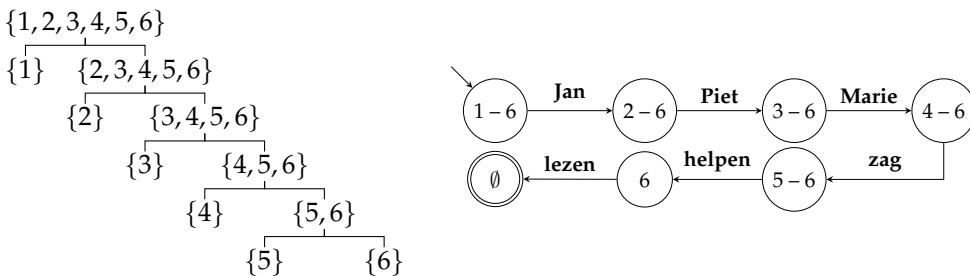
Figure 13 A right-branching recursive partitioning and an FA.
