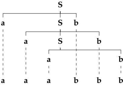
Figure 5 Abstract representation of cross-serial dependencies in Dutch as discontinuous phrase structure.
