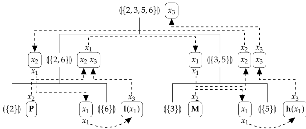
Figure 18 Derivation tree for the recursive partitioning of Figure 17, induced by the sDCP rules.
