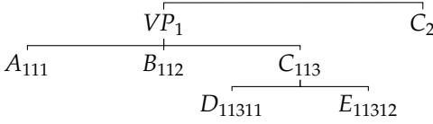
Figure 3 Illustration of the s-term \langle VP(\langle A(\langle \rangle), B(\langle \rangle), C(\langle D(\langle \rangle), E(\langle \rangle)) \rangle)), C(\langle \rangle) \rangle where positions are annotated in subscript at each node.
