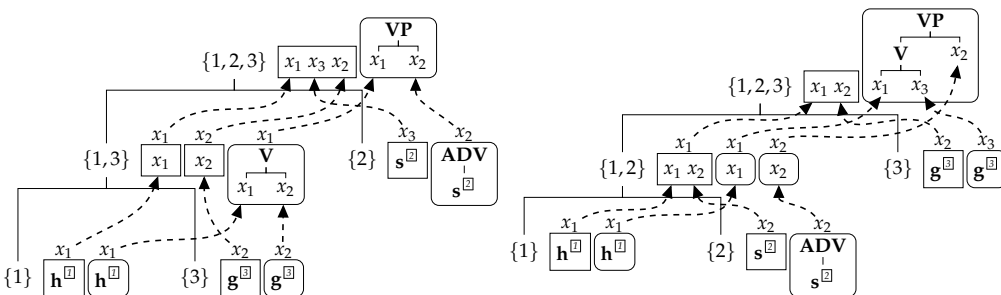
Figure 16 (Left) The only derivation tree of the LCFRS/sDCP hybrid grammar induced in Example 19 with the recursive partitioning extracted from the hybrid tree. (Right) The only derivation tree of the LCFRS/sDCP hybrid grammar induced in Example 20 with the left-branching recursive partitioning.
