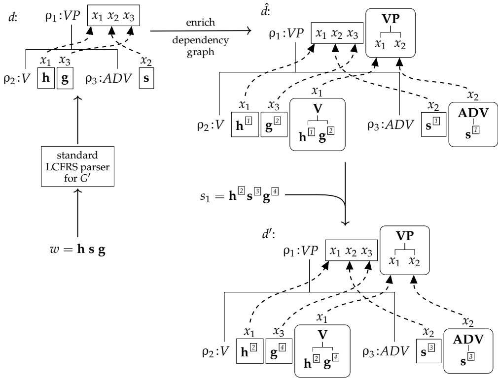
Figure 9 Algorithm 1 applied to the LCFRS/sDCP hybrid grammar G from Example 11 and the sentence w = h s g .
