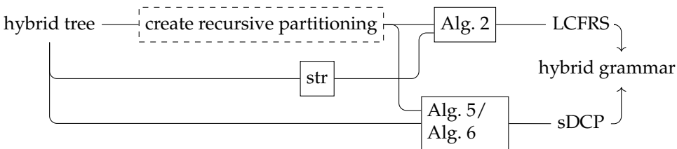
Figure 14 Pipeline for the induction of LCFRS/sDCP hybrid grammars.
