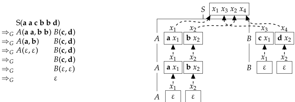
Figure 6 Derivation and derivation tree of the LCFRS in Example 7.
