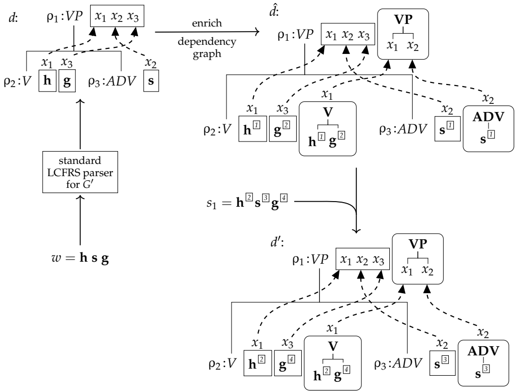
Figure 9 Algorithm 1 applied to the LCFRS/sDCP hybrid grammar G from Example 11 and the sentence w = h s g .
