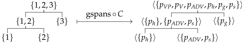
Figure 15 The left-branching recursive partitioning of \{1, 2, 3\} and the image under \text{gspans} \circ C .
