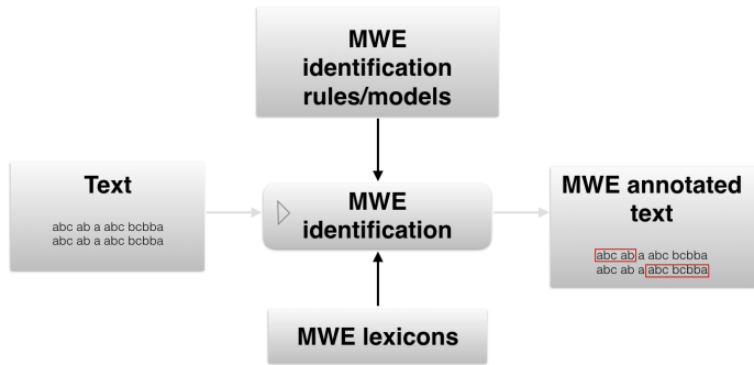
Figure 3 MWE identification: find occurrences of MWEs in running text.
