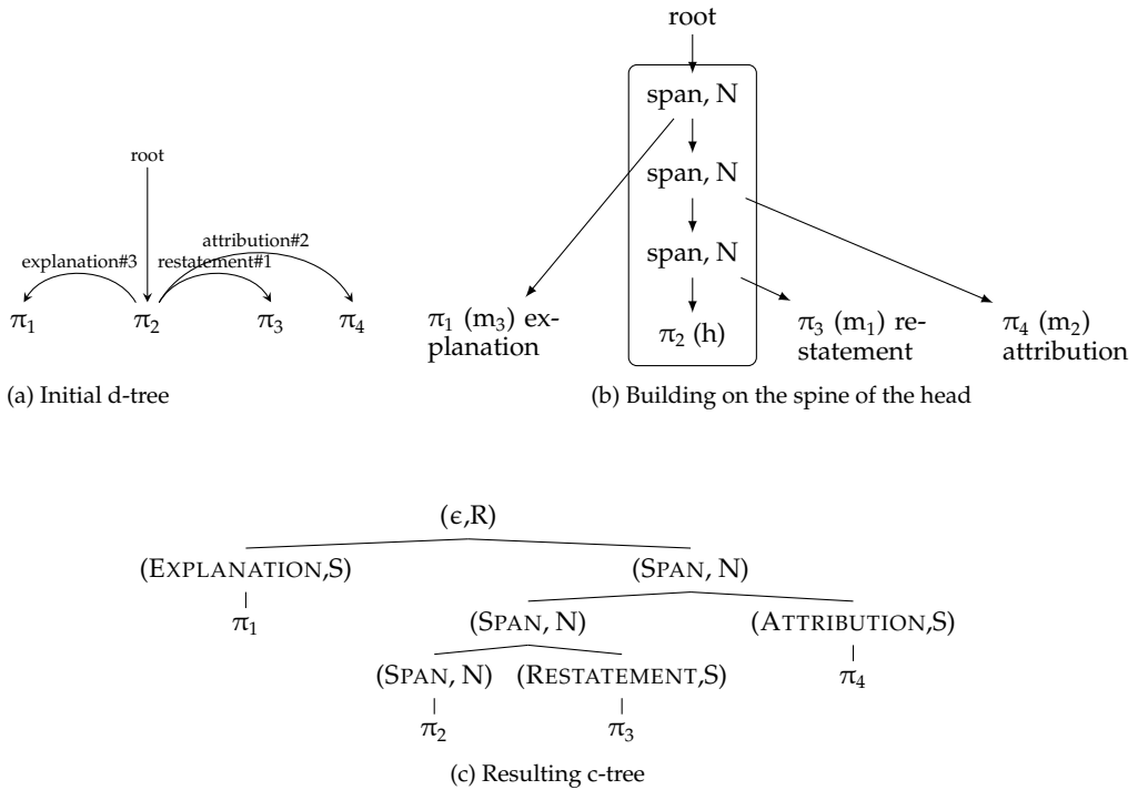
Figure 7 Transformation of a strictly ordered RST d-tree (a) into a binary RST c-tree (c) using the order of attachment (b).
