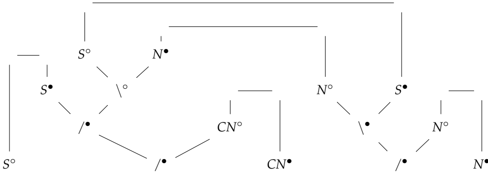
Figure 2 Proof net: The parsing structure of categorical grammar (Morrill 2000).
